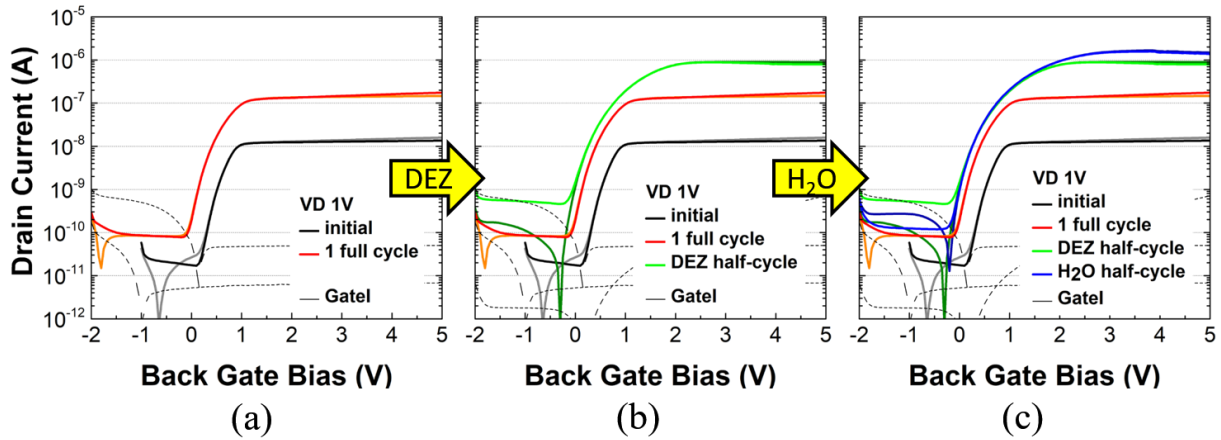
Figure 2. Half-cycle study of I_{DS} - V_{GS} transfer curves of inverted-coplanar structured ZnO TFT. Transfer curve of (a) 45 ZnO ALD cycles (initial, black) and 46 ZnO ALD cycles (1 full cycle, red), (b) after DEZ half-cycle (green), and (c) after H_2O half-cycle (blue).
