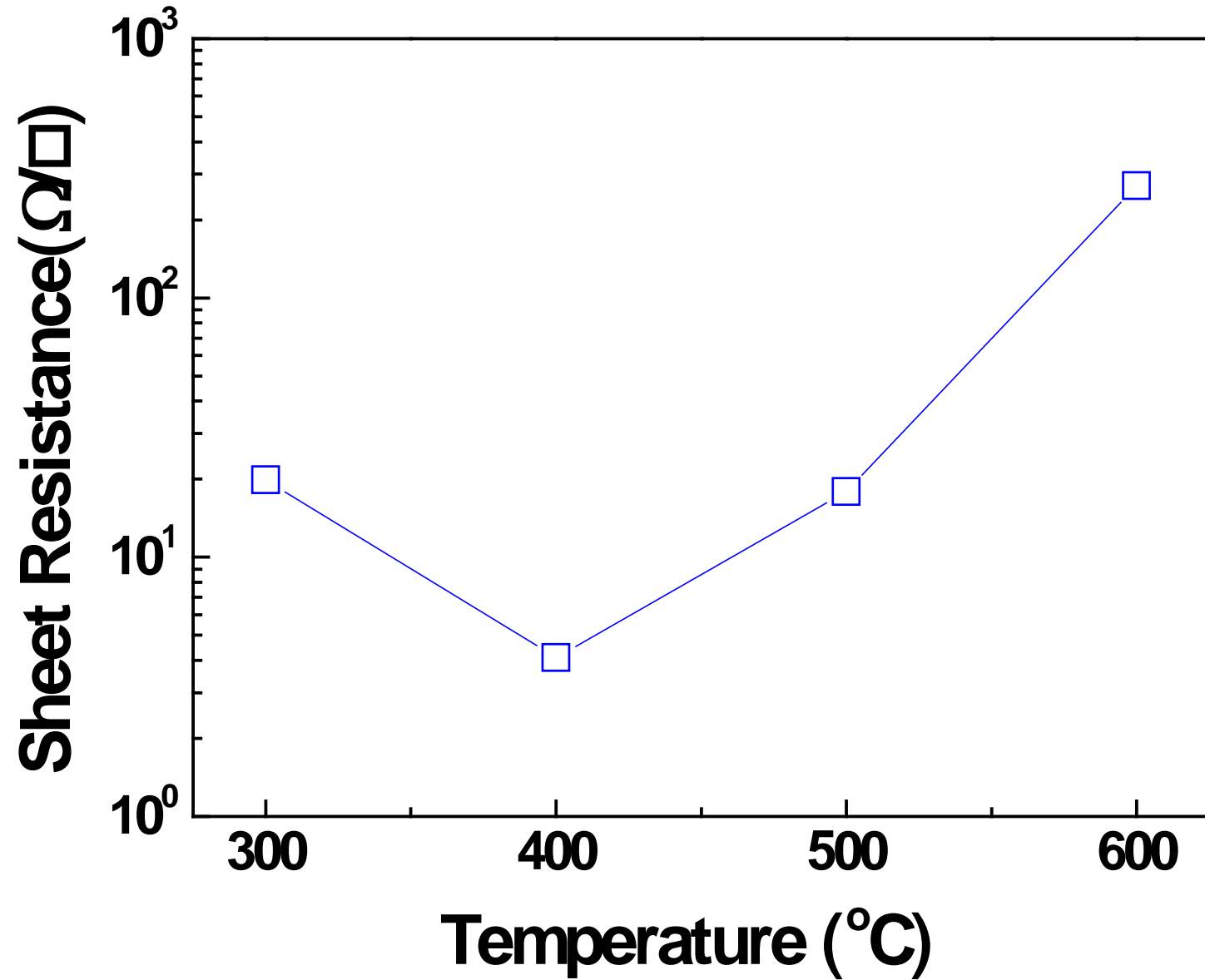
Fig 1. Sheet resistance of Ni-GeSn samples annealed at various temperatures for 60 seconds
