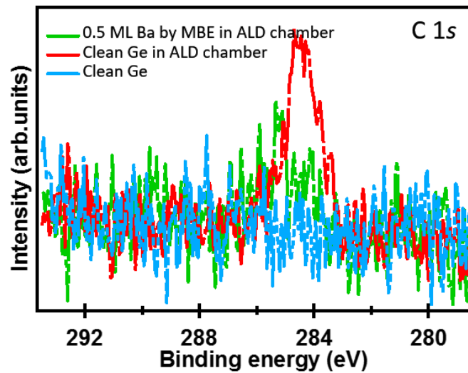
Figure 2. C 1s X-ray photoelectron spectra of clean Ge, clean Ge that was moved into the ALD chamber for 15 mins, and a 0.5-ML Ba on Ge surface that was moved into the ALD chamber for 15 mins.
