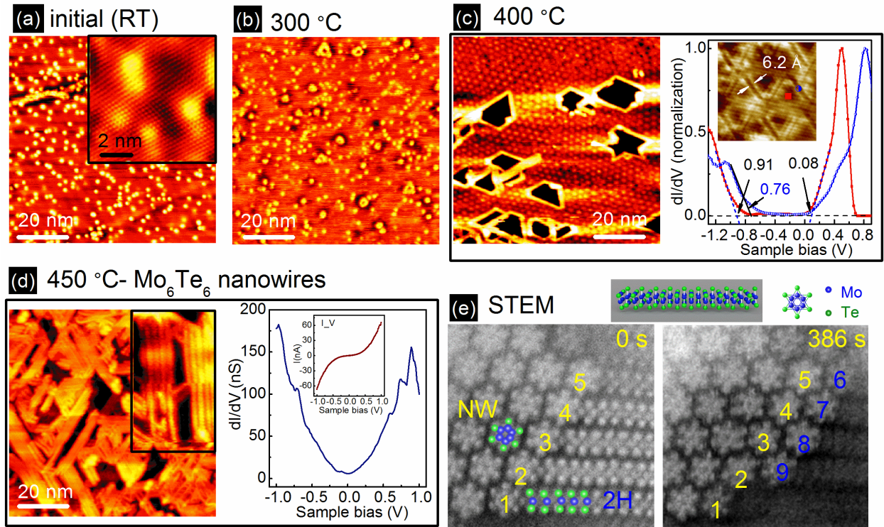
Figure S1. Structural stability and phase transition of \text{MoTe}_2 under vacuum annealing.
