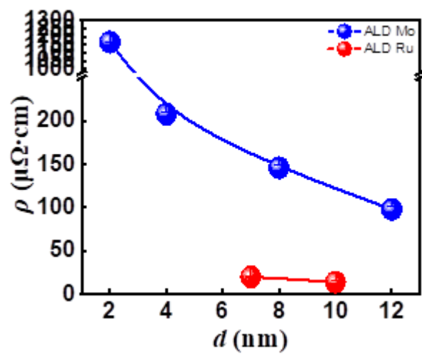
Fig. 2. ALD Mo and Ru Resistivity
