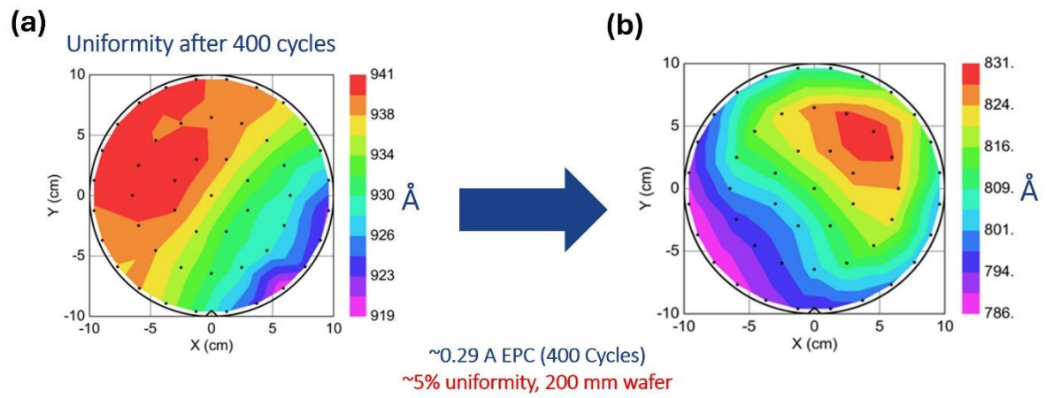
Fig. 1: 200 mm wafer mapping of nominally undoped ZnO. (a) As grown and (b) after 400 cycles of ALE.
