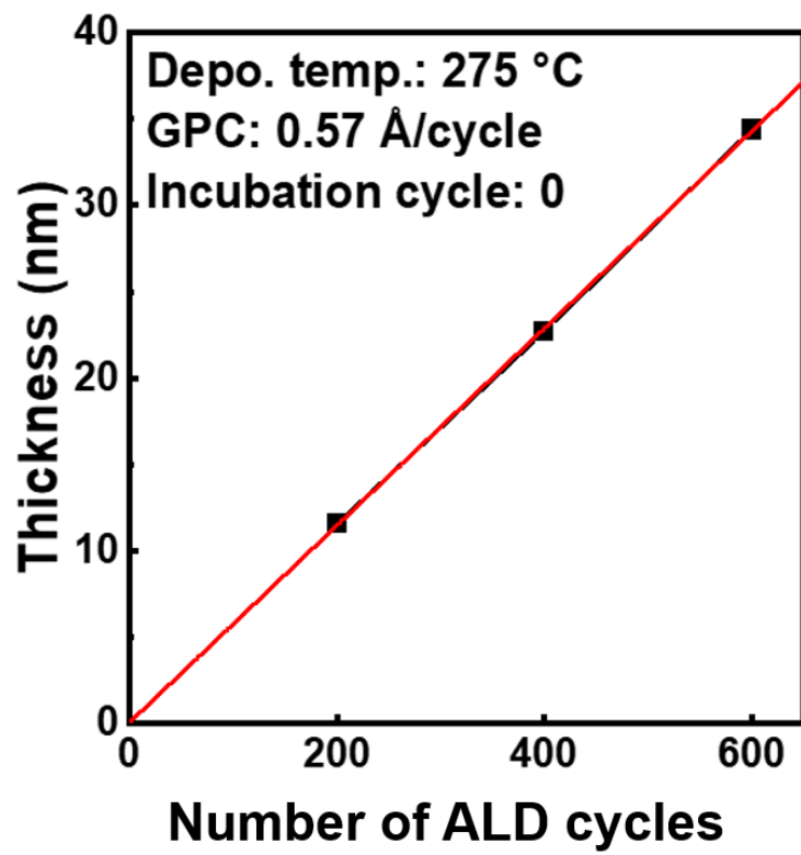
Figure 1. ALD-grown InN film thickness as a function of the number of ALD cycles at 275 °C
