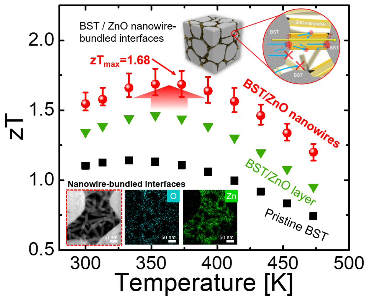
Fig 1. Schematic of enhancing Figure of merit via nanowire-bundled grain boundaries
