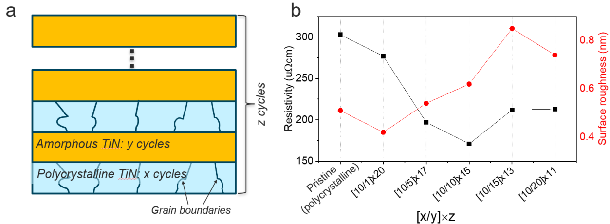
Figure S1. Multilayer thin film composes of alternating amorphous and polycrystalline TiN layers. a) schematic structure of the multilayer, b) Electrical resistivity and surface roughness (RMS) of ~10nm thin films.
