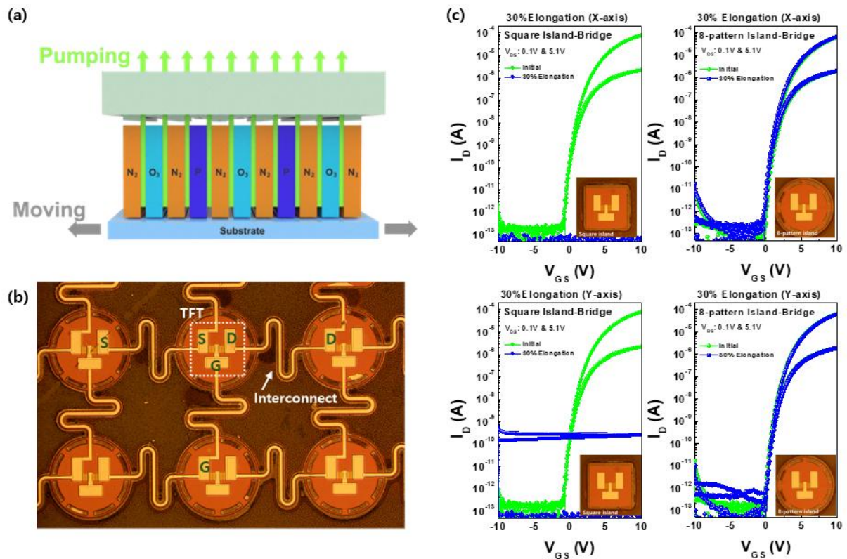
Figure 1. (a) Schematic of AP S-ALD method (b) Optical Microscope image of 8 pattern island-bridge structured IZO TFT (c) Schematic of x and y-axis elongation of island-bridge structured TFT transfer curve (square, 8 pattern) under 30% elongation
