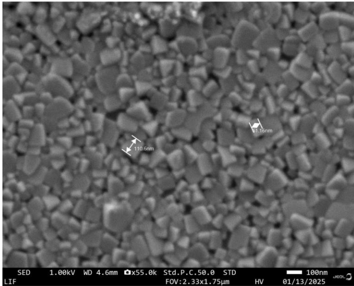
Figure 1: SEM image of a 62 nm LiF film
