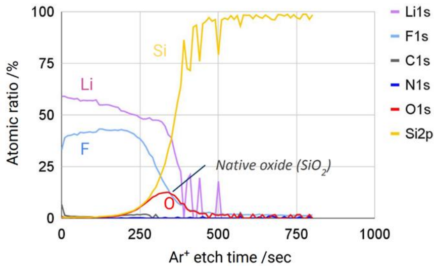
Figure 2: XPS spectrum of LiF on a silicon substrate
