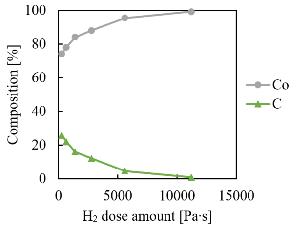
Figure 3. Co film composition versus H 2 dose amount.
