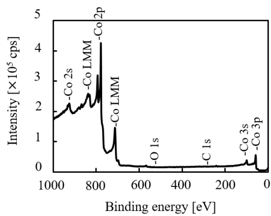
Figure 4. The XPS spectrum of Co film.
