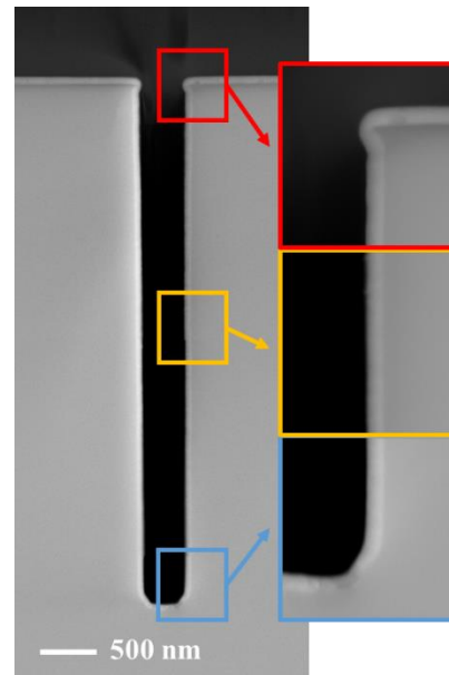
Figure 2. The SEM image of Co film on trench structure.
