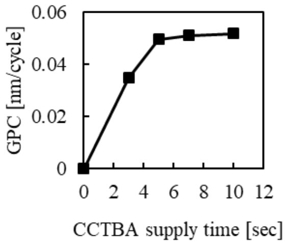
Figure 1. GPC versus CCTBA supply time.
