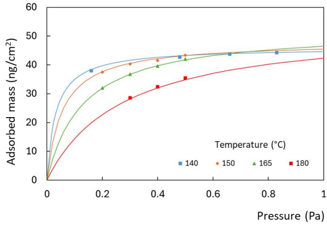
Fig. 1 Chemisorbed mass of TMA by in-situ QCM with various temperatures and TMA partial pressures
