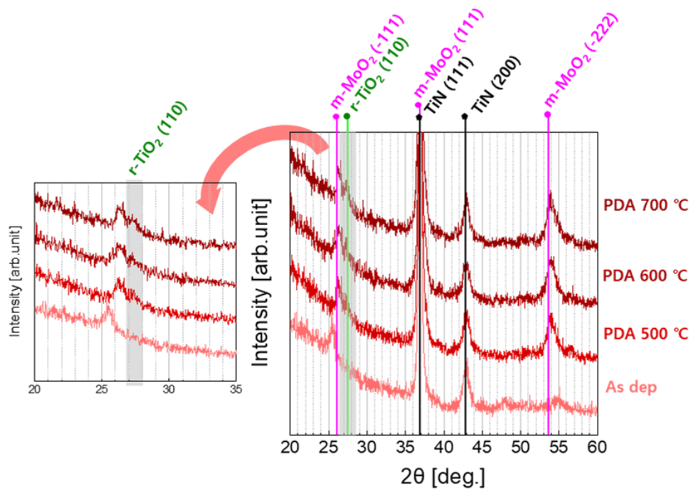
Fig 2. XRD patterns of the ALD TiO 2 films on as-deposited and annealed ALD MoO 2 films on TiN.
