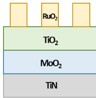
Fig 1. A Schematic of metal-insulator-metal structure.
