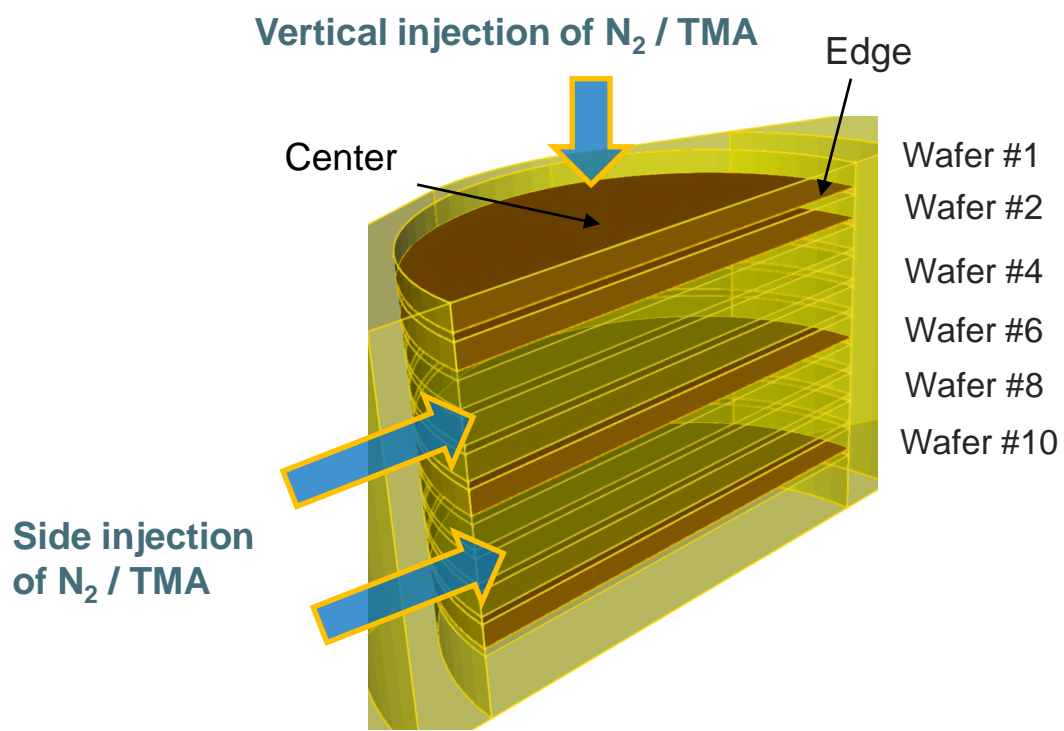
Fig.1. 3D geometry of batch ALD reactor
