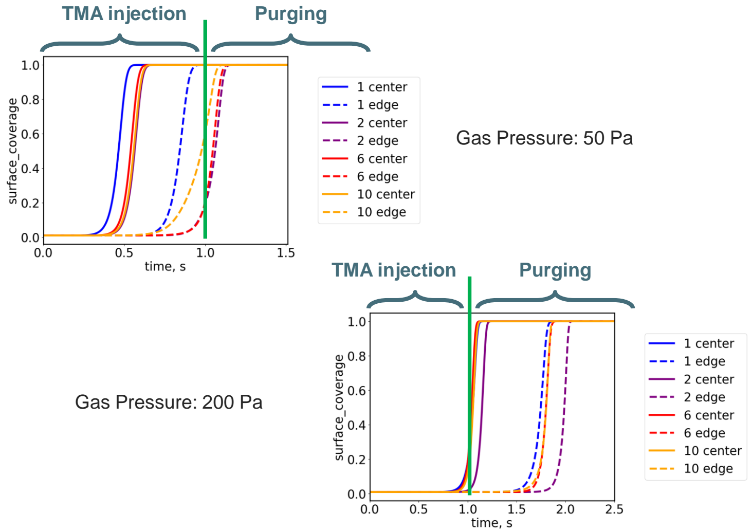
Fig. 2. Surface coverage as a function of time during TMA precursor delivery and purging steps.
