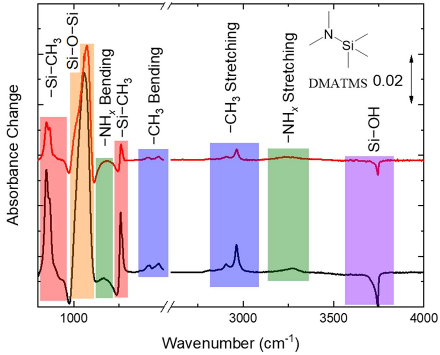
Figure 2. In situ IR spectrum of DMATMS adsorption on SiO 2 with (red) and without (black) a pre-anneal at 500 °C.
