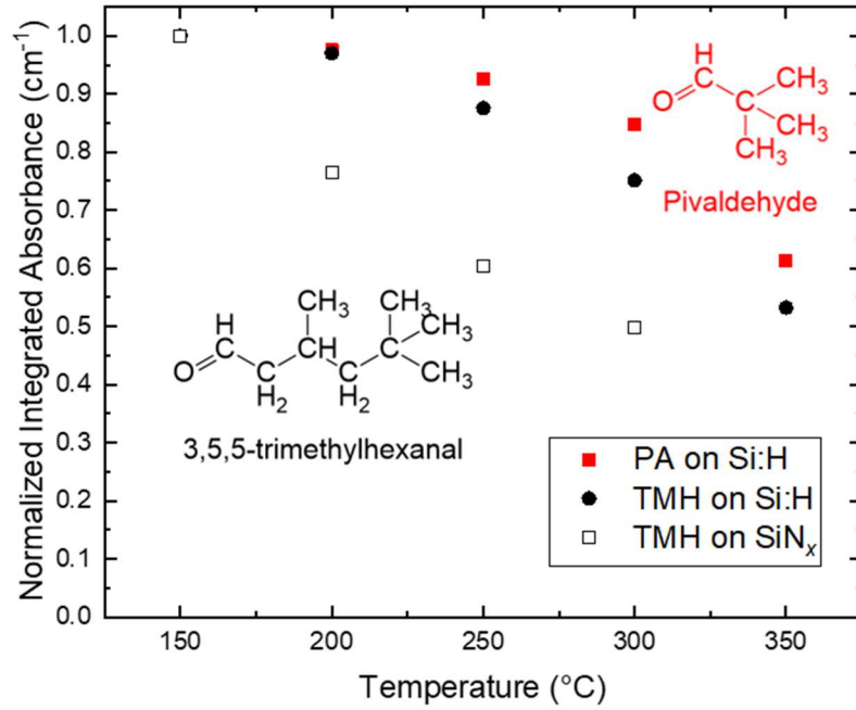
Figure 1. Thermal stability of pivaldehyde on Si:H and SiN x , and TMH on SiN x .
