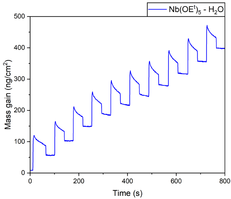
Figure 2: QCM mass change measured during Nb(OE t ) 5 -H 2 O ALD process, on uncoated crystal (bare Cr/Au electrode)
