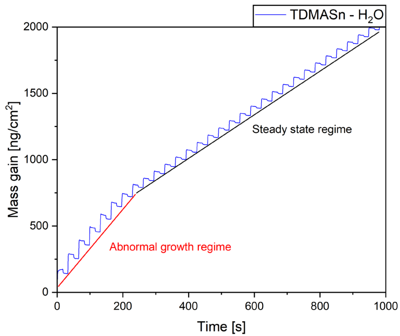
Figure 1: QCM mass change measured during TDMASn-H 2 O ALD process, on uncoated crystal (bare Cr/Au electrode)
