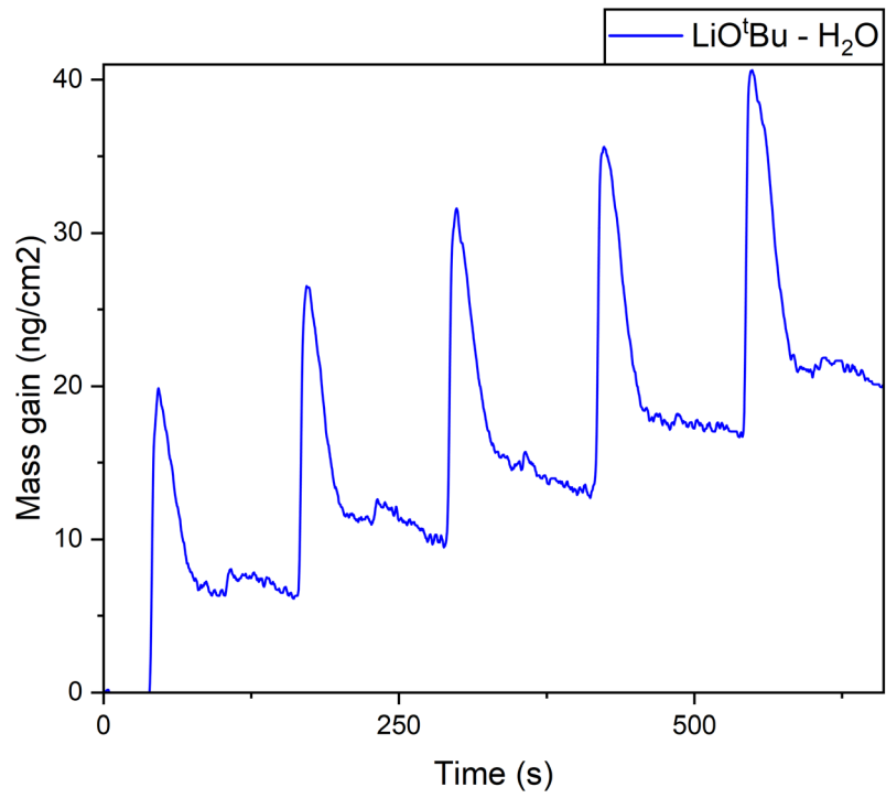
Figure 3: QCM mass change measured during LiO t Bu-H 2 O ALD process, on uncoated crystal (bare Cr/Au electrode)
