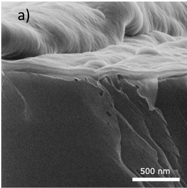
Figure 1. a) Cross section of 500 cycles of Al 2 O 3 using TMA and water on cellulose fiber. b) Cross section of ALD ZnO film with 10 nm Al 2 O 3 adhesion layer grown on inconel powder that has been prepared by milling with neon beam.
