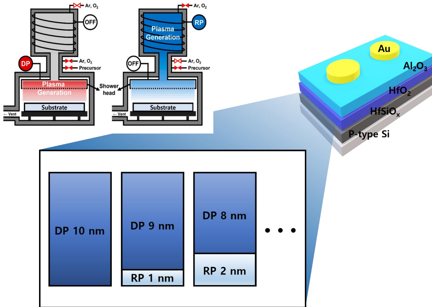
[Schematic Diagram of Charge Trapping Memory by Sequential Plasma Atomic Layer Deposition]
