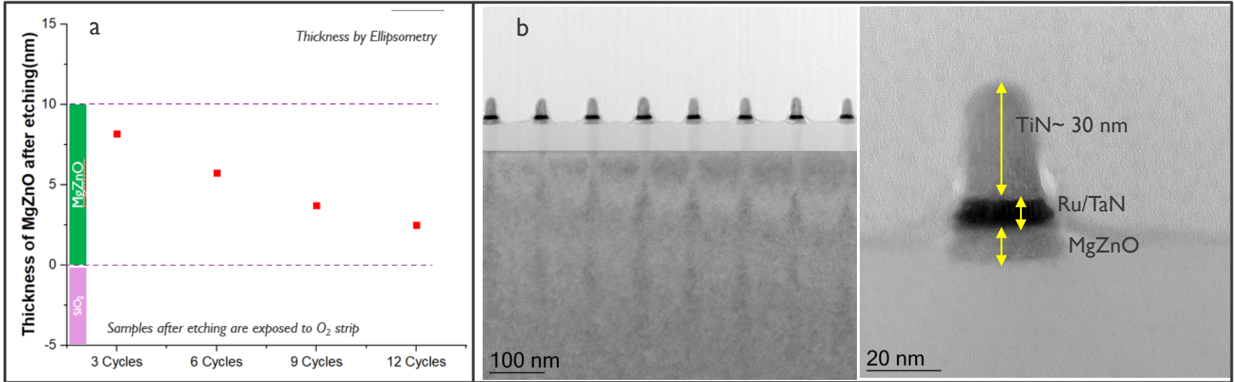
Fig 1: a) Thickness of blanket MgZnO after ALE cycles, b) TEM images of MgZnO on the pattern after 9 cycles of ALE
