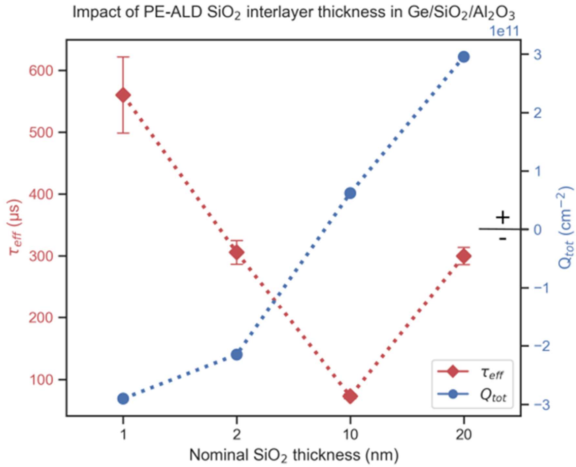
Figure 1: \tau_{eff} and Q_{tot} of Ge samples with 20 nm ALD Al 2 O 3 film as function of PE-ALD SiO 2 interlayer thickness. Samples were annealed 30 min at 400 °C after ALD.
