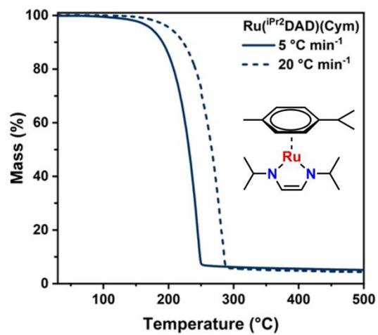
Figure 1: Thermogravimetric analysis of Ru( i Pr 2 DAD)(Cym) recorded with different heating rates.
