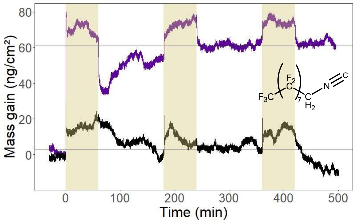
Figure 1: QCM adsorption experiment of C9 on gold (purple trace) and alumina (black trace) at 100 °C. Shaded regions are 1-hour exposures of C9 and unshaded regions are 2-hour purges.
