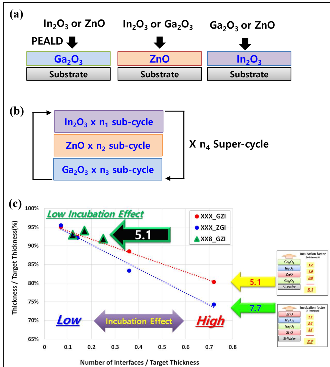
Fig. 2. Illustrations of incubation experiments for (a) oxide films with different substrate and (b) multilayer IGZO. (c) Thickness control of the films with different incubation factor
