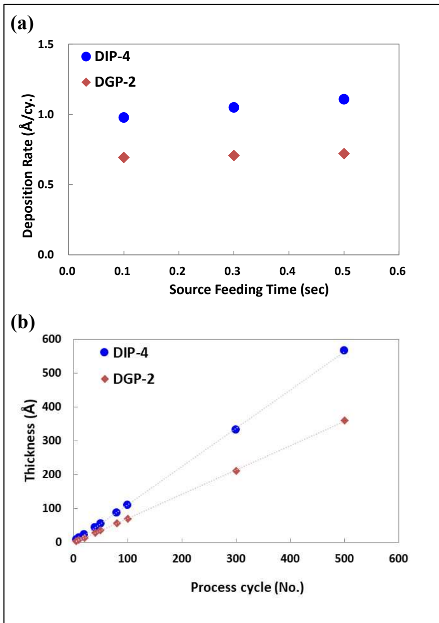
Fig. 1. (a) source feeding time saturation and (b) linearity of indium oxide and gallium oxide
