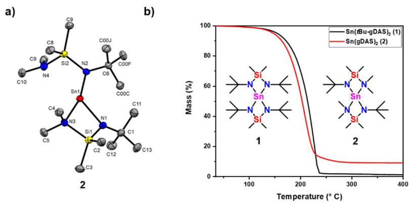
Figure 1. a) Crystal structure of [\text{Sn}(\text{gDAS})_2] ( 2 ). b) TGA of compounds [\text{Sn}(\text{tBu-gDAS})_2] ( 1 ) and [\text{Sn}(\text{gDAS})_2] ( 2 ) revealing promising volatilization.
