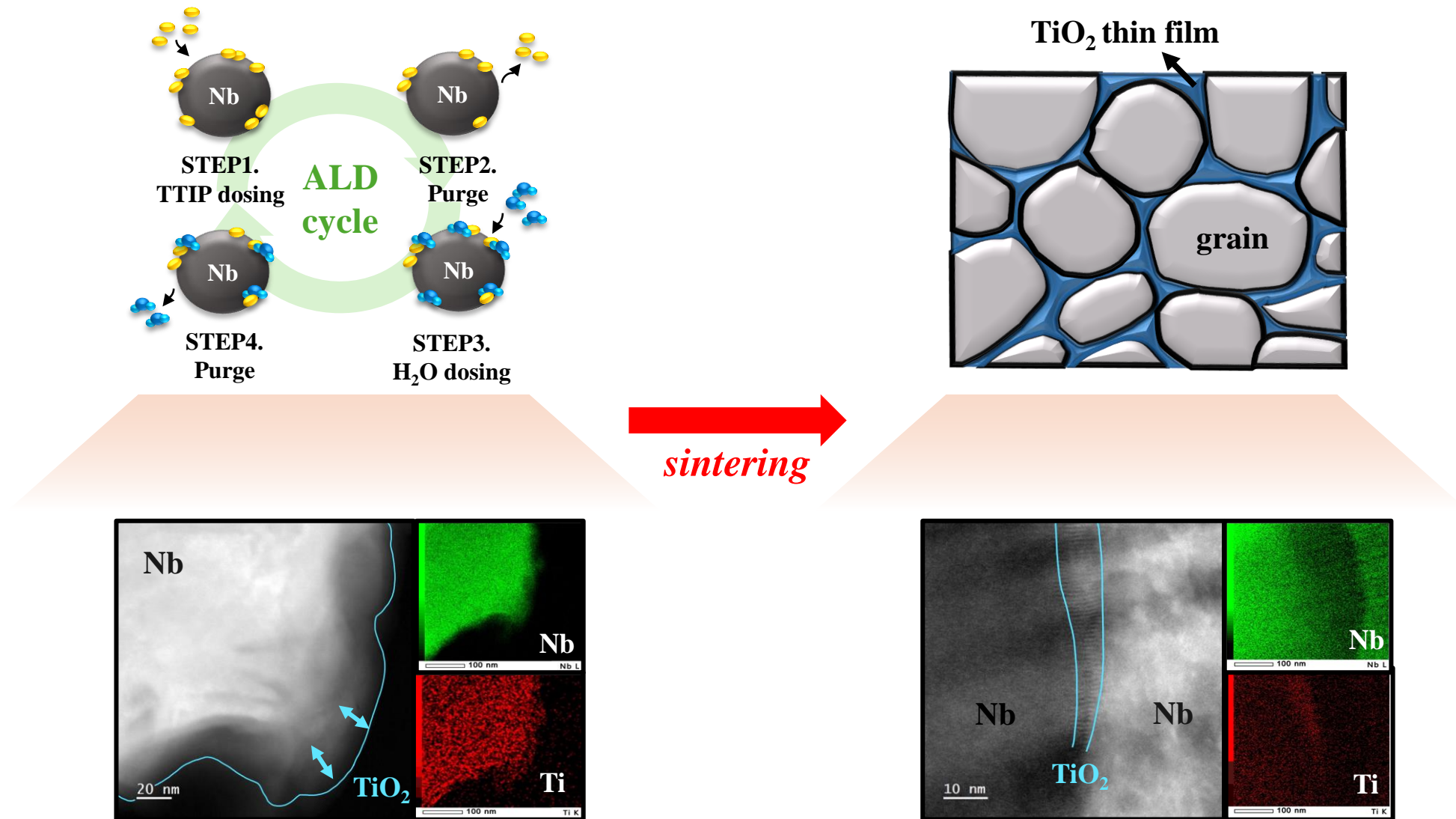
Fig. 1. A schematic of the ALD process on Nb powders and sintered pellets. The corresponding STEM images and EDS mapping results are shown below.
