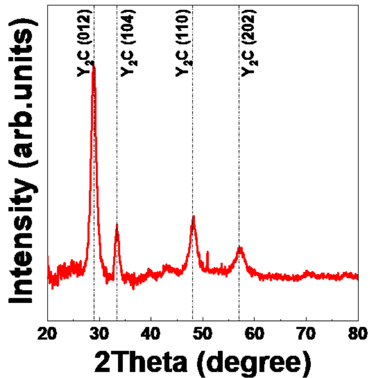
Figure 2. The XRD peak of yttrium carbide at 250 degrees.
