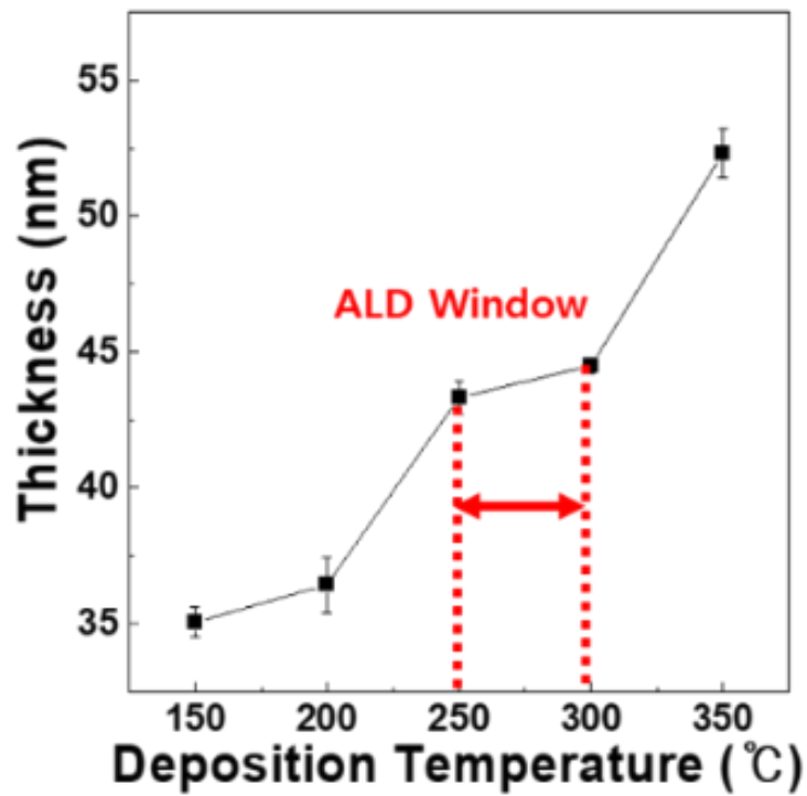
Figure 1. The ALD window range of yttrium carbide thin films
