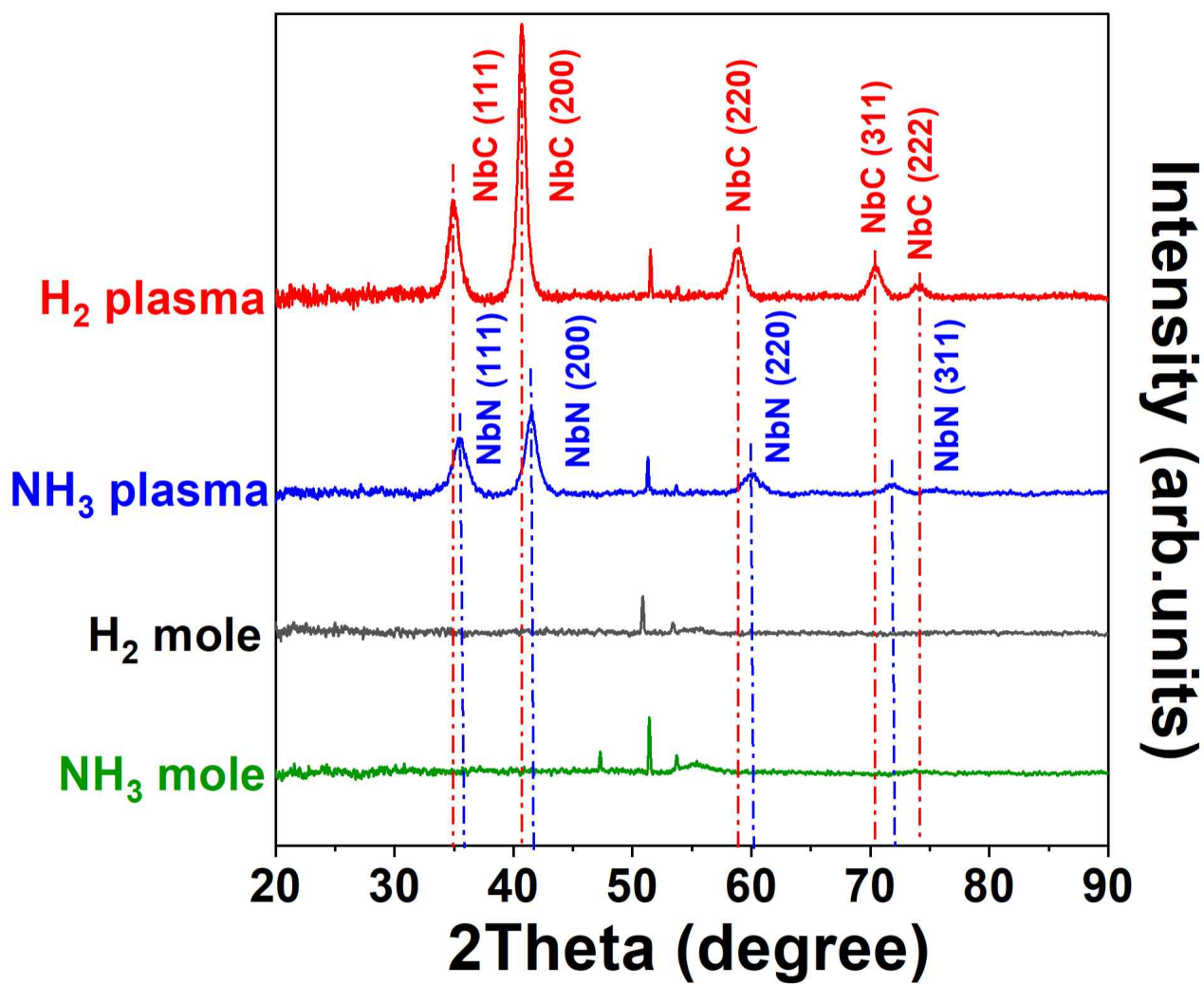
Figure 1. X-ray diffraction (XRD) patterns of various reactants
