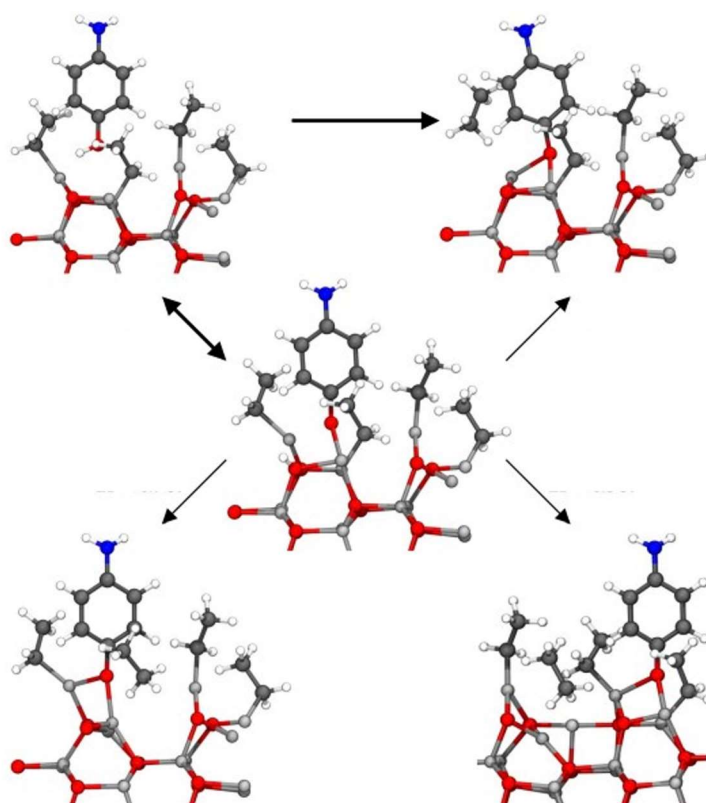
Figure 2: Hydrogen migration from the hydroxyl group of 4-Aminophenol to ethyl ligand utilizing both ligand exchange and dissociation reactions to grow the hybrid thin film.
