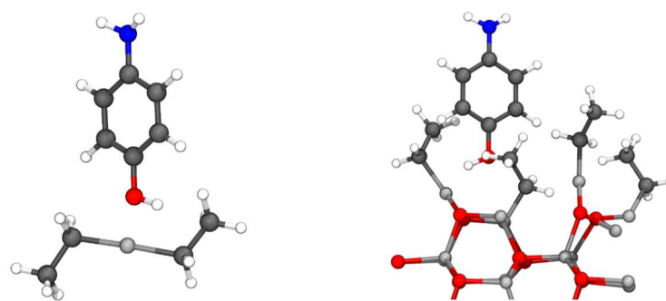
Figure 1: Initial state of a hybrid thin film growth reaction in gas-phase (left) and surface model (right).
