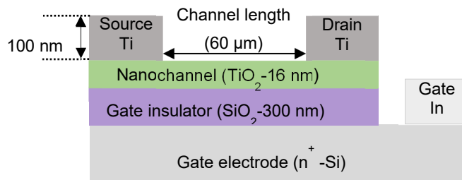
Fig.1 TiO 2 thin film transistor for monitoring the RT TiO 2 ALD.
