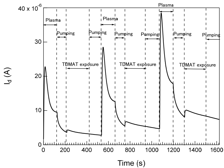
Fig.3 Drain current waveform measured by a nanothick TiO 2 TFT during the TiO 2 RT-ALD.
