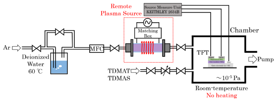
Fig. 2 RT TiO 2 ALD system with the monitoring TFT.
