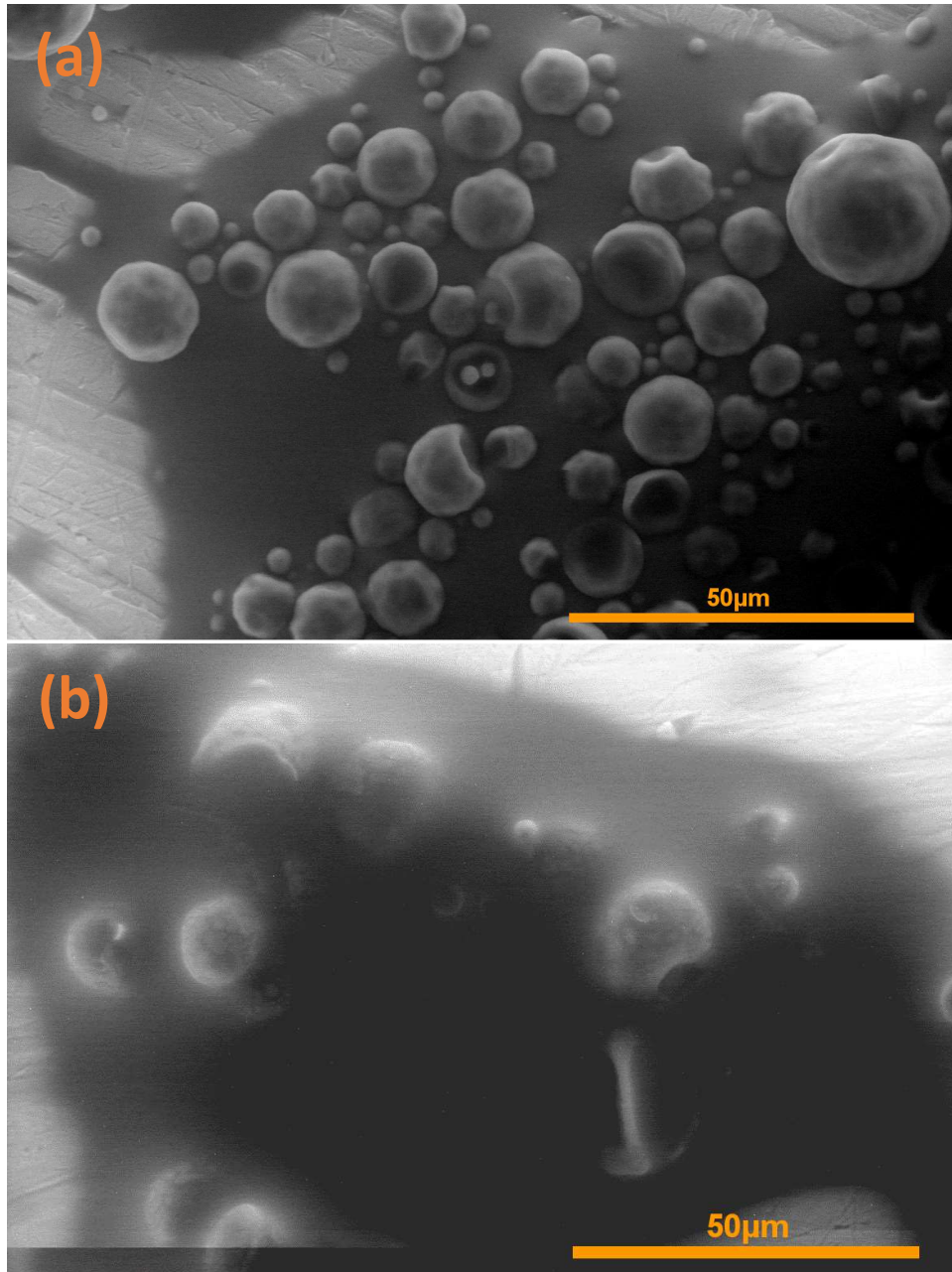
Figure 1. ESEM images of (a) pristine sample and (b) sample subjected to 1 deposition cycle of SiO 2 in the presence of moisture
