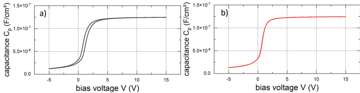
Figure 2. a) Capacitance-voltage of PP/SiO 2 b) Capacitance-voltage of best-know-method PP/SiO 2
