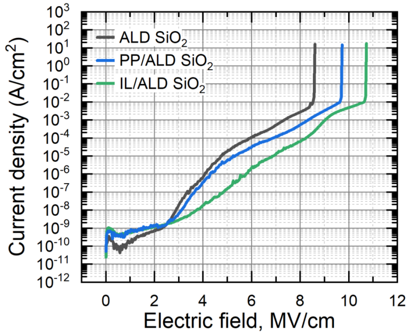
Figure 1. Current-voltage characteristics of ALD SiO 2 on 4H-SiC.
