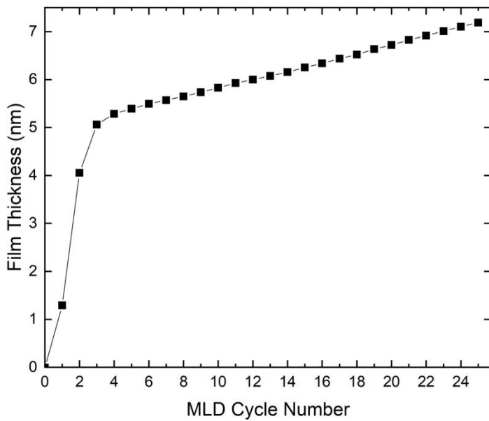
Figure 2: Thickness of DICB/DETA film throughout 25 cycles of MLD, measured by in situ ellipsometry.
