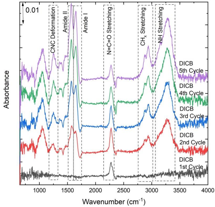
Figure 1: Infrared spectra of DICB/DETA film throughout 5 cycles of MLD, with reference spectrum collected prior to each cycle.
