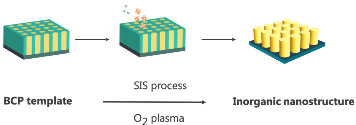
Figure 1. Illustration of HfO x nanostructure fabrication process using block copolymer (BCP) as template via sequential infiltration synthesis (SIS).
