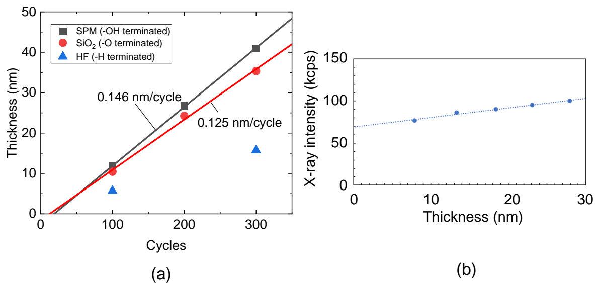
Fig. 2: (a) Ru film thicknesses of three different surfaces and (b) calibration curve between X-ray intensity and thickness of Ru film.
