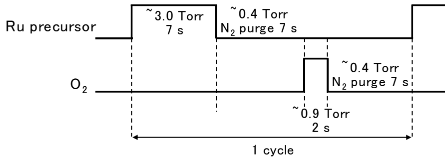
Fig. 1: schematic time sequence of Ru ALD.
