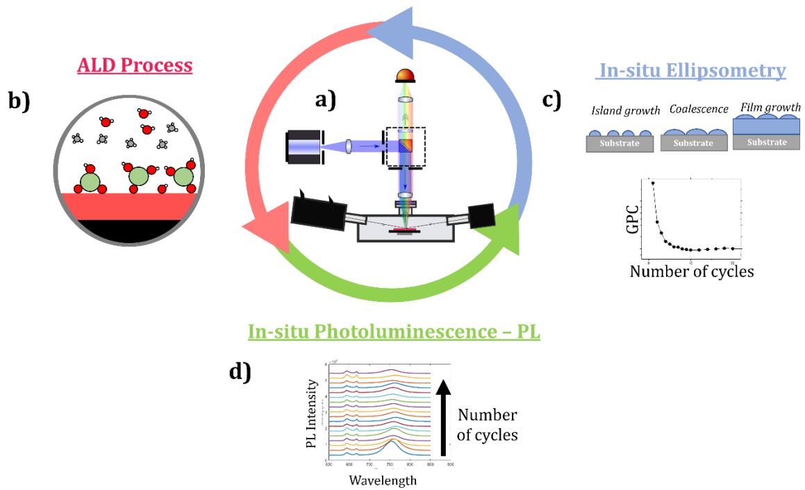
Fig. 1 a) Experimental set-up with in-situ PL and ellipsometry in an ALD reactor b) ALD growth c) In situ ellipsometry - Thickness, optical constants and growth mechanisms d) In situ PL – Functionalization properties (passivation, carrier behaviour)
