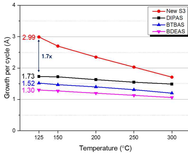
Fig 1. Growth-per-cycle of O 2 plasma-enhanced ALD using a novel and conventional Si precursors
