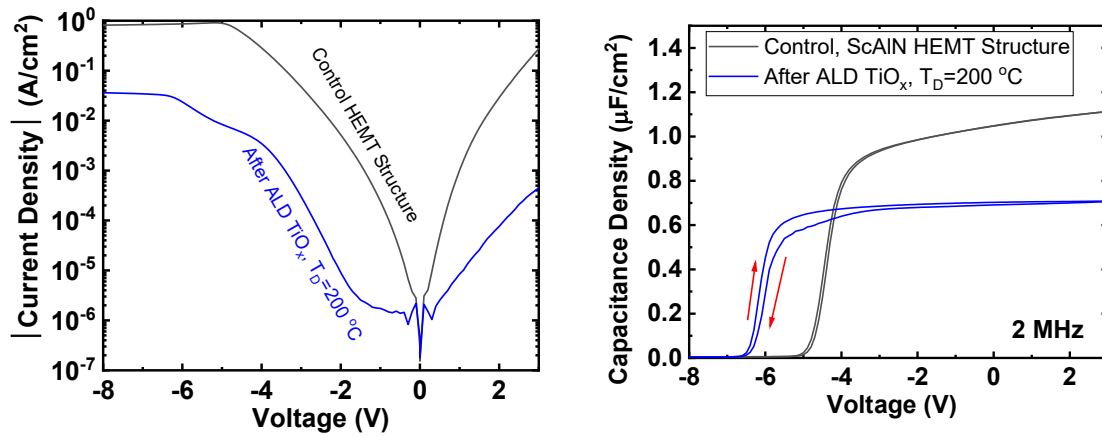
Fig. 2 Vertical I-V and C-V of ScAlN HEMT structure with Schottky contact (black line) compared to structure with ALD TiO 2 (blue line).
