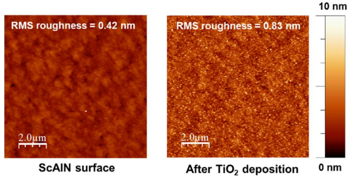
Fig. 1 AFM images of ScAlN surface of ScAlN HEMT structure before and after TiO 2 deposition.
