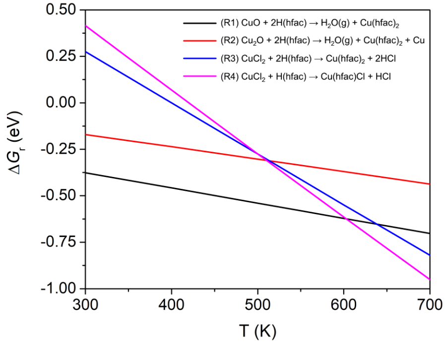
Fig.1 Gibbs free energies of the reactions between H(hfac) and CuO, Cu 2 O, and CuCl 2 at different temperatures.
