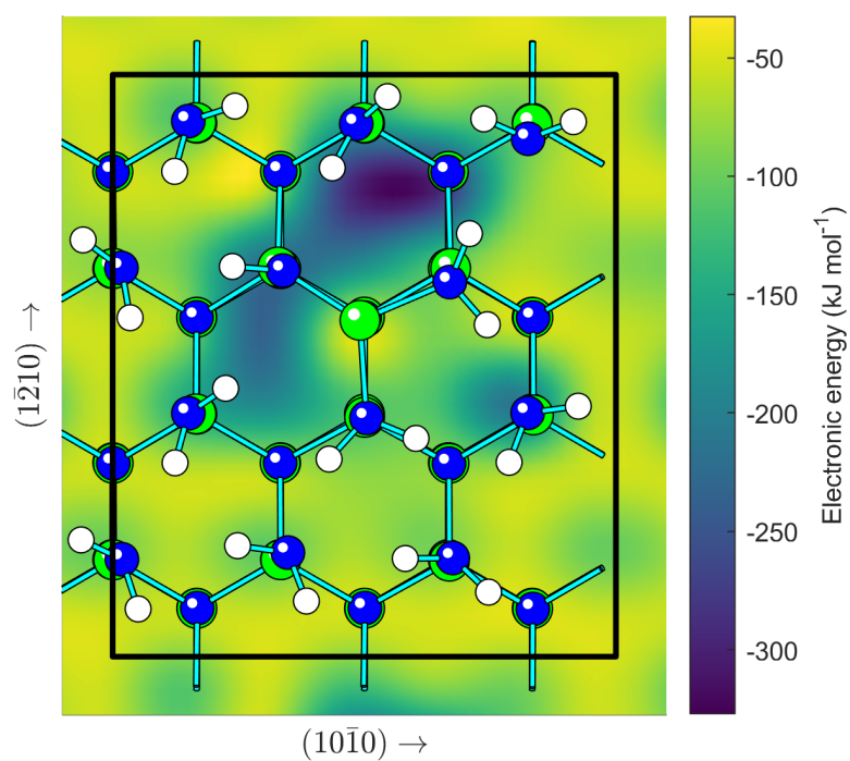
Figure 2. Potential energy surface for a TMA-molecule adsorbing onto a NH 2 -terminated AlN surface with an aluminum atom previously deposited.
