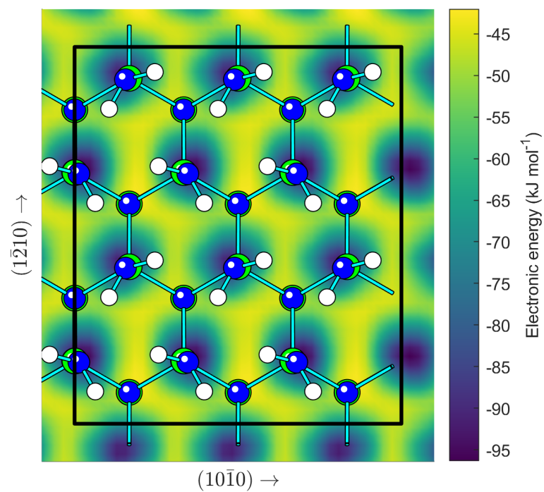
Figure 1. Potential energy surface for a TMA-molecule adsorbing onto an empty NH 2 -terminated AlN surface.
