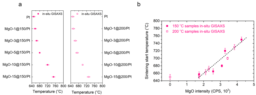
Figure 2. (a) Sintering onset temperature for two group of samples. (b) Sintering onset temperature as the function of Mg signal intensity extracted from XPS.
