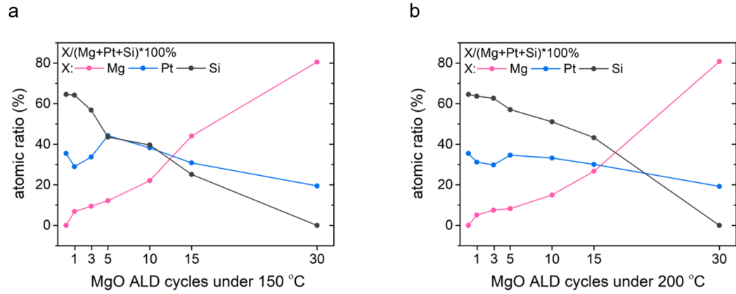
Figure 1. Elemental ratio evolution as the function of ALD cycles under (a) 150 °C and (b) 200 °C.
