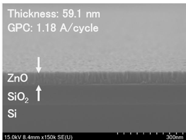
Fig.2: ALD growth zinc oxide film on SiO 2 substrate using ZNP-2 & H 2 O at 200°C.
