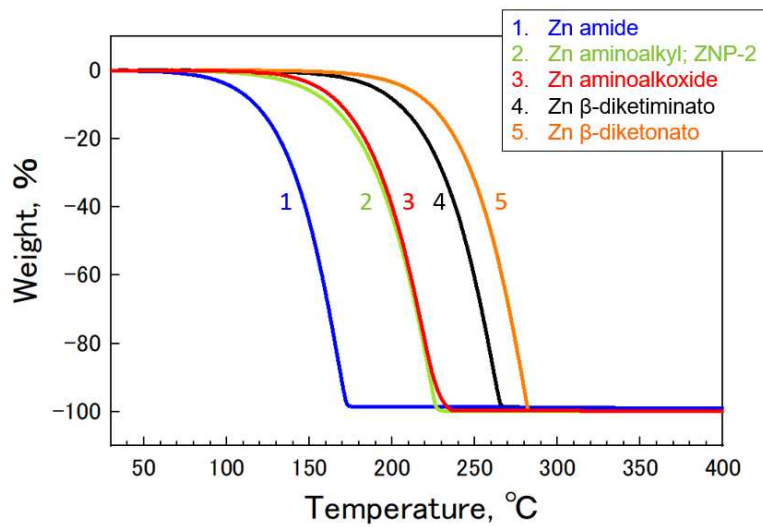
Fig.1: TGA spectra of various kinds of volatile zinc molecules including ZNP-2 (under 760 torr)
