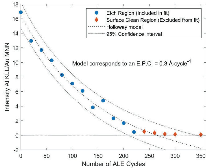
Figure 2 – AES intensity ratios for Al KLL and Au MNN as a function of number of ALE cycles at 250°C. Blue circles designate the Etch Region using model from Holloway. Orange diamonds designate the Surface Clean Region .
