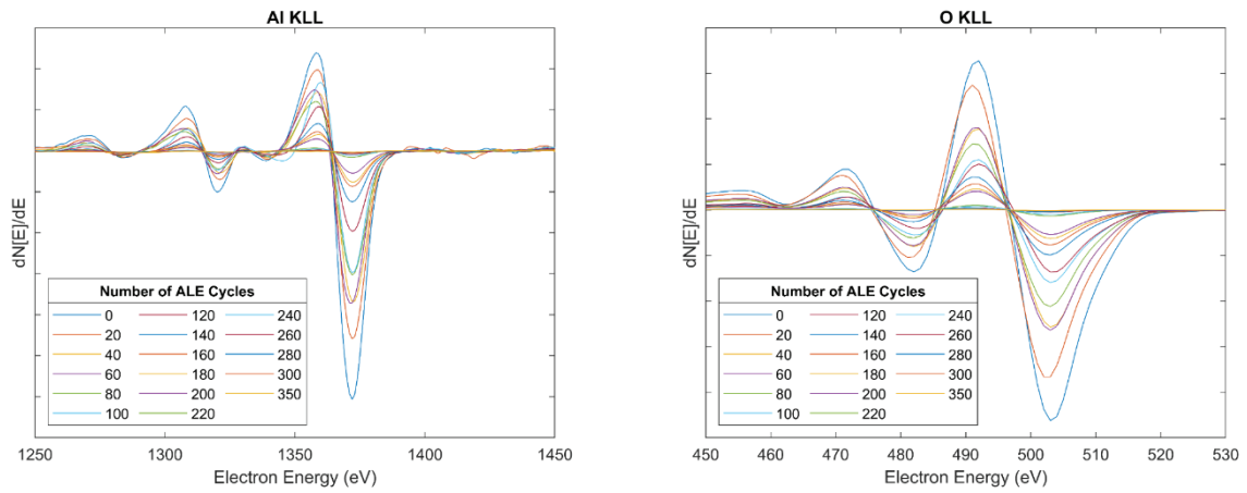
Figure 1 – AES peaks for Al KLL (left) and O KLL (right). Peaks were normalized to their respective Au substrate peaks in each scan.
