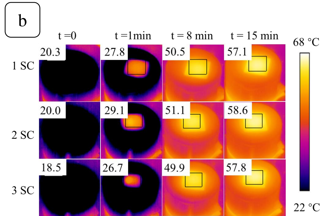
Figure 1: (a) Extinction spectra of silver-silica hybrid films with different thickness and (b) photothermal effect produced by different layer thicknesses as a function of time.
