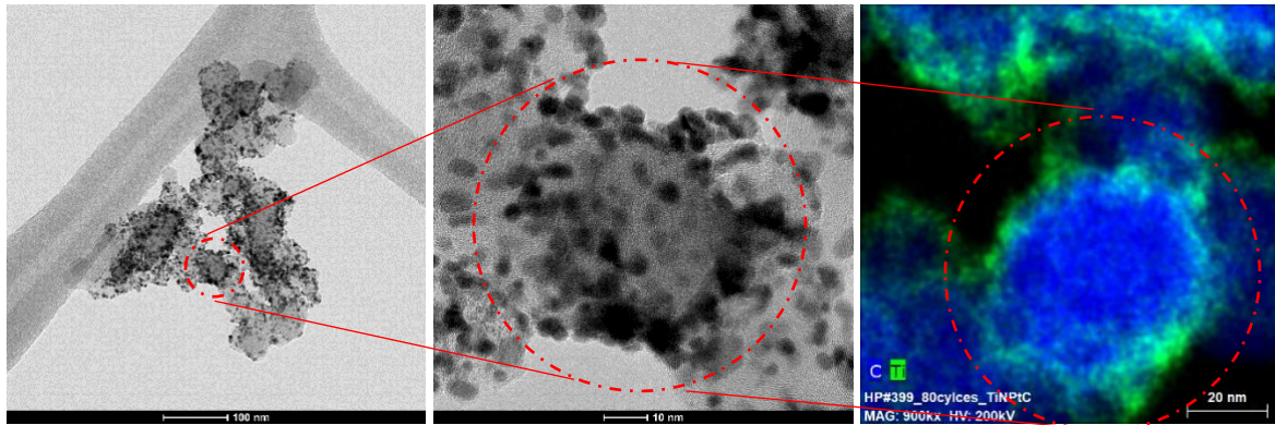
Figure 1. HR-TEM imaging and EDS mapping of Pt (black on Bright field TEM)/C(gray on Bright field TEM and blue on EDS map) and Ti (green EDS map) after 80 ALD cycles.
