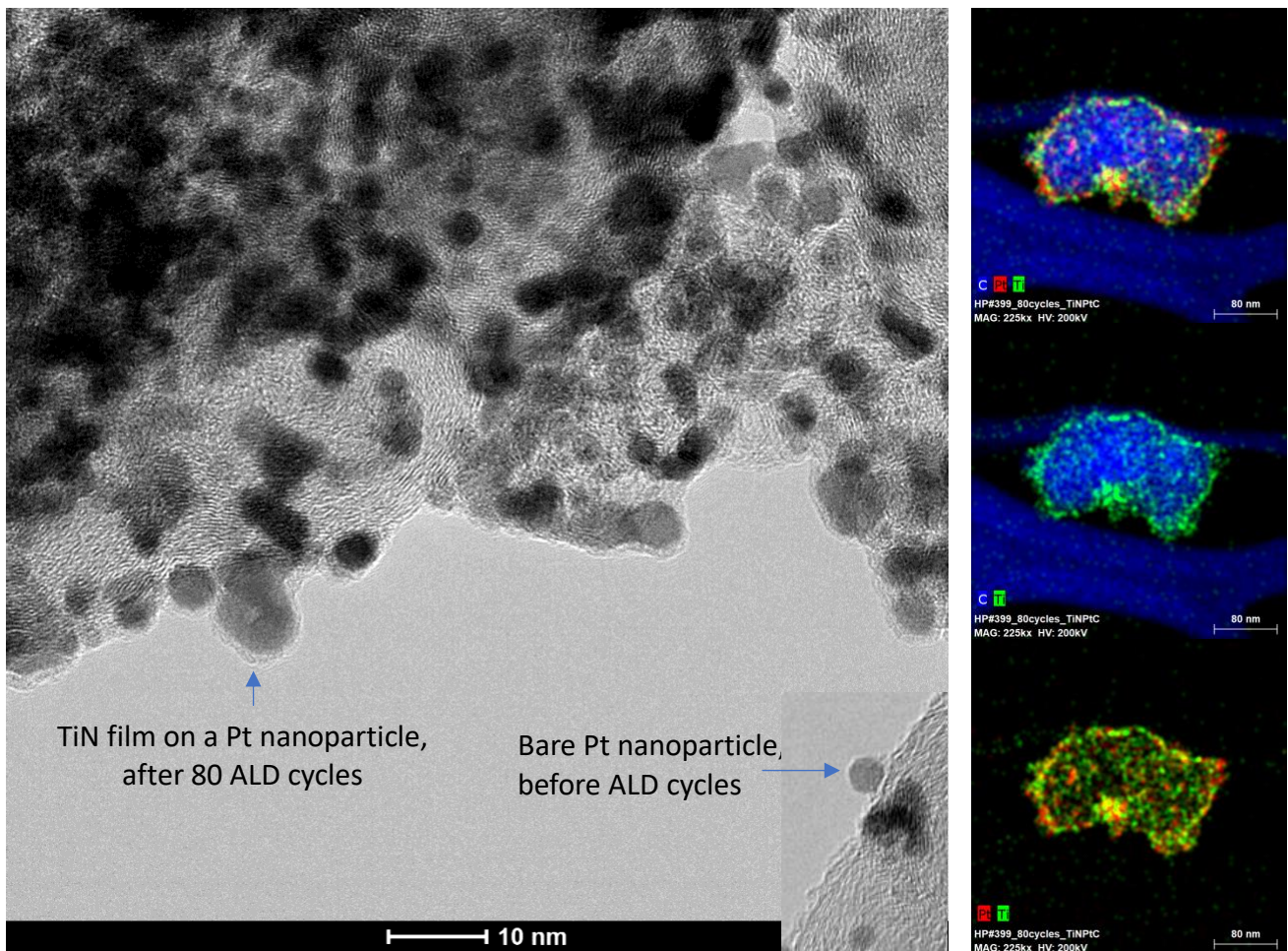
Figure 2. HR-TEM imaging and EDS mapping of Pt/C covered by TiN.
