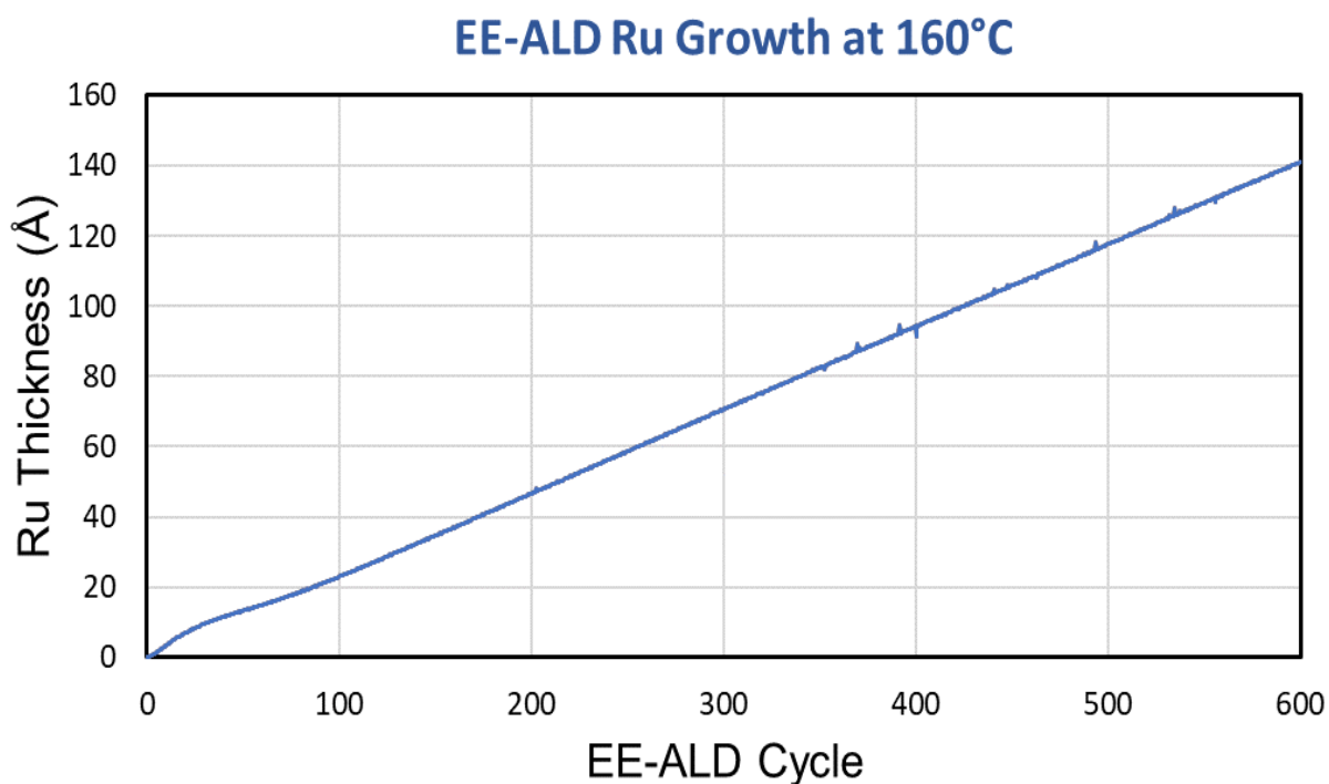
Figure 2: In-situ spectroscopic ellipsometry of Ru grown at 160°C using (DMBD)Ru(CO) 3 and electrons.
