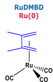
Figure 1: Sequential surface reactions for Ru EE-ALD and (DMBD)Ru(CO) 3 precursor.
