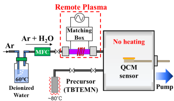
Fig.1 Schematic of RT-ALD system with QCM sensor.
