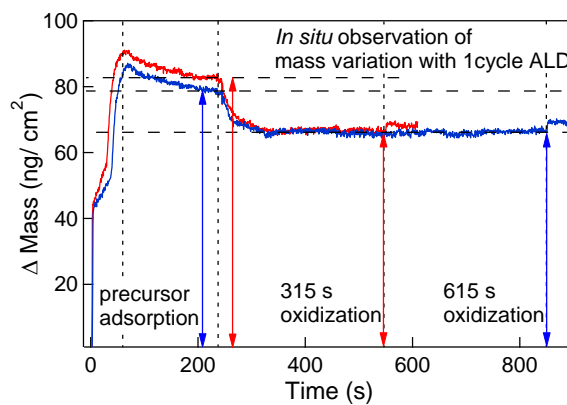
Fig.2 Quartz crystal surface mass variation in the one cycle of Nb 2 O 5 RT-ALD. Redline indicates in case of 315 s oxidization, and blue is case of 615 s.
