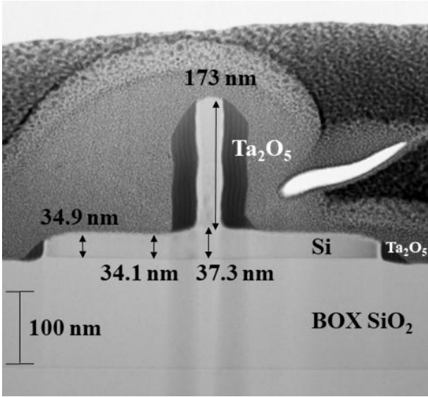
Figure 1: Illustration of a Ta 2 O 5 topographically selective deposition (TSD) on sidewalls of a 3D structure.
