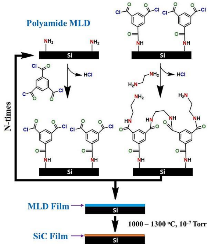
Figure. Synthesis of SiC films by heat treatment of MLD polyamide film on Si
