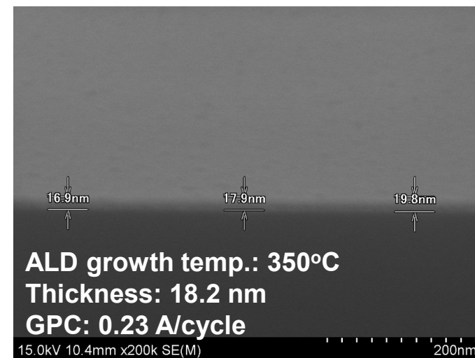
Figure 2: FE-SEM image of HfO 2 film
