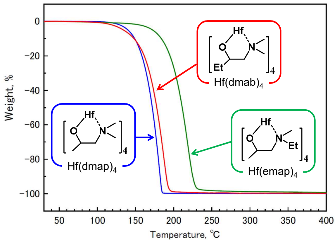
Figure 1: TGA of Hafnium aminoalkoxide precursors (10 torr)
