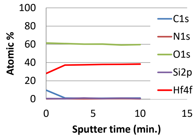
Figure 3: XPS depth profile of HfO 2 film (375°C)
